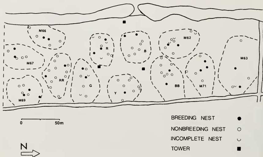
FIG. 1. Territories of 12 male Sedge Wrens during the week beginning 9 July, when most females were beginning their second clutches.
